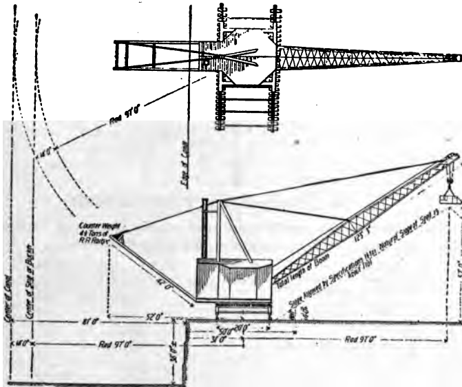
Fig. 157. Hullett-McMyler Derrick.
